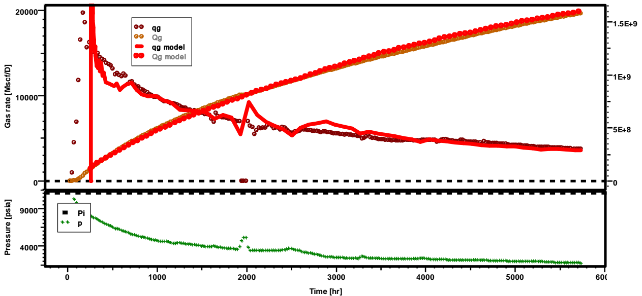
History match with the analytical model after nonlinear regression
