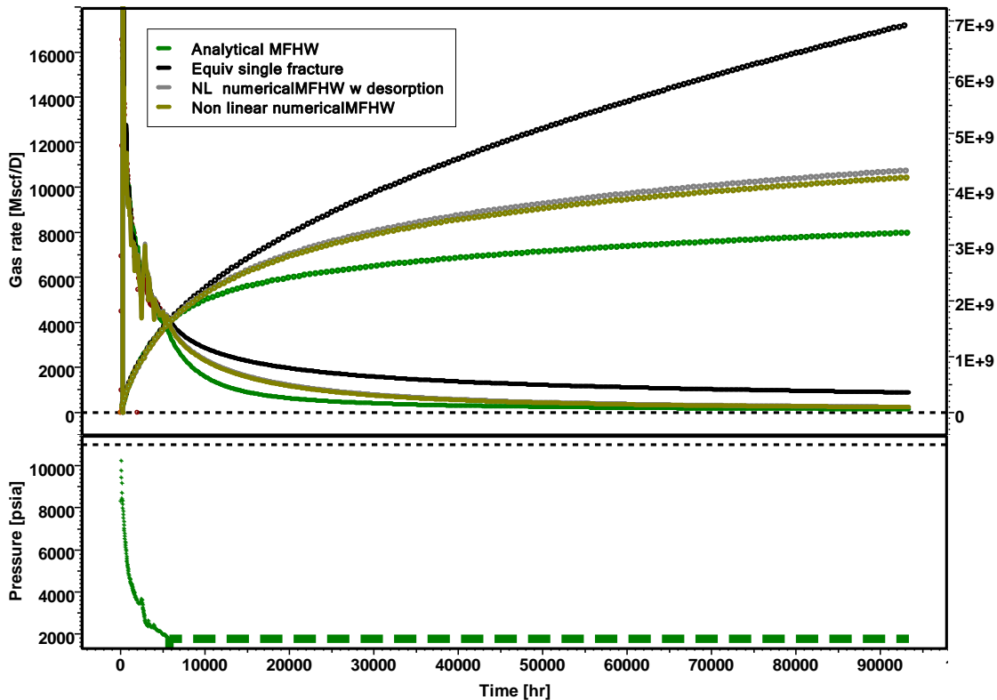
Comparison of 10-year forecasts
