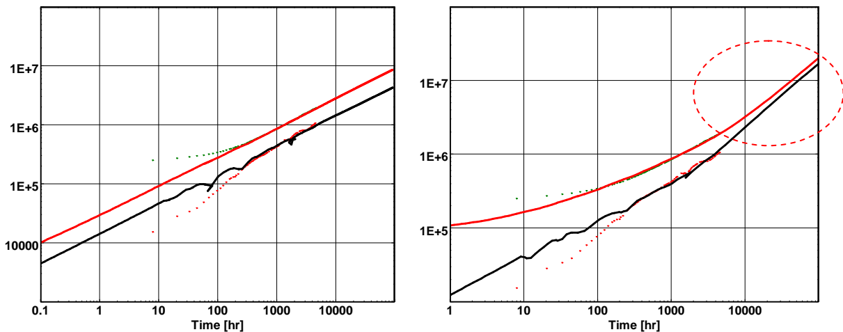
Comparison of the loglog response for both straight line and analytical models
