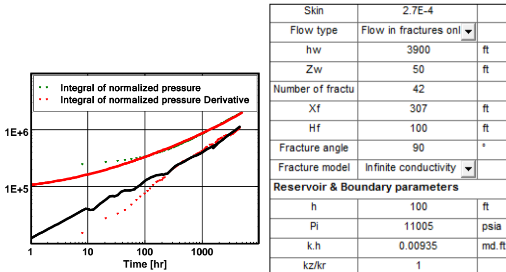
Loglog match and analytical model parameters after nonlinear regression
