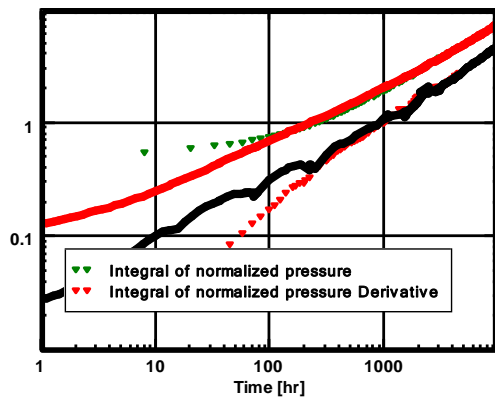
History match, loglog match, and model parameters
