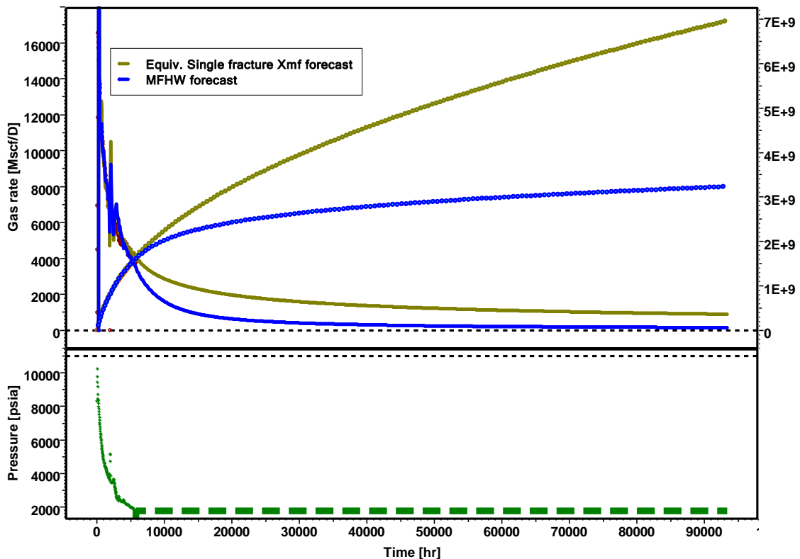
Comparison of forecast for both straight line and analytical models
