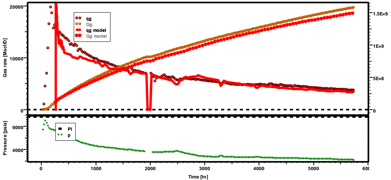
History match using the analytical model with the straight line result.
