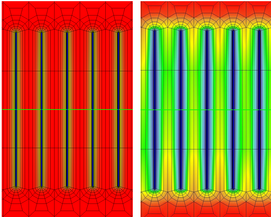
Pressure field after one month and 8 months
