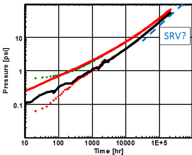
Log-log plot after 10-year forecast
