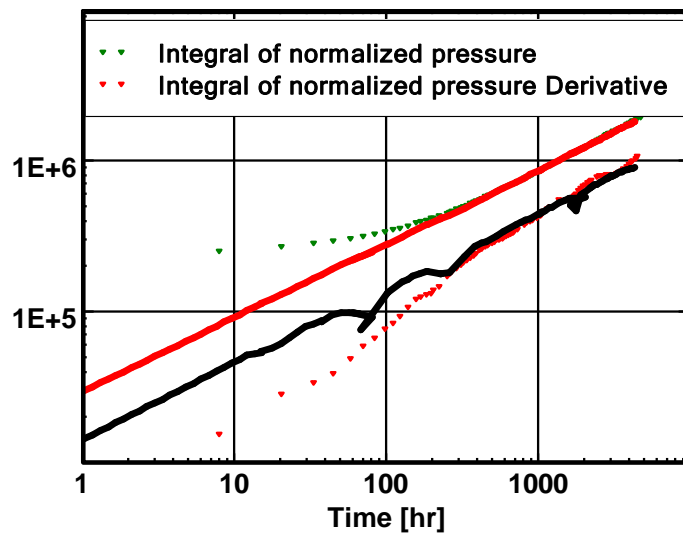
History and Loglog match
