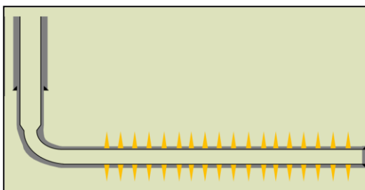
Well completion schematic
