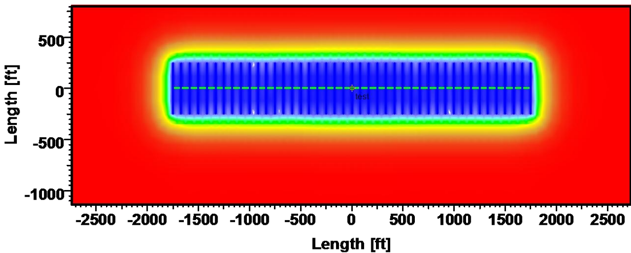
After 10-years of production (forecast)
