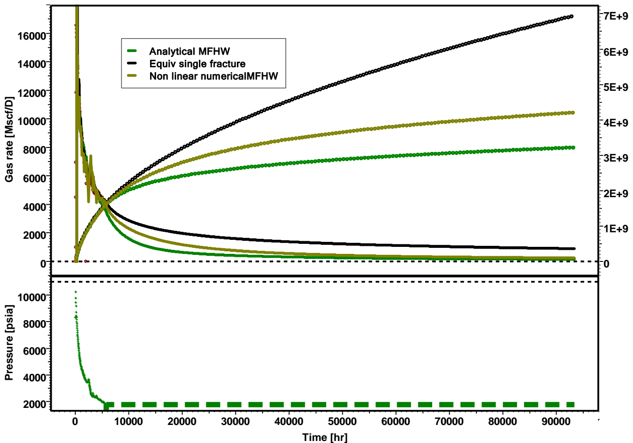
Comparison of 10-year forecasts
