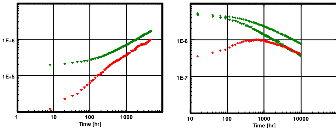
History plot, log-log plot and Blasingame plot
