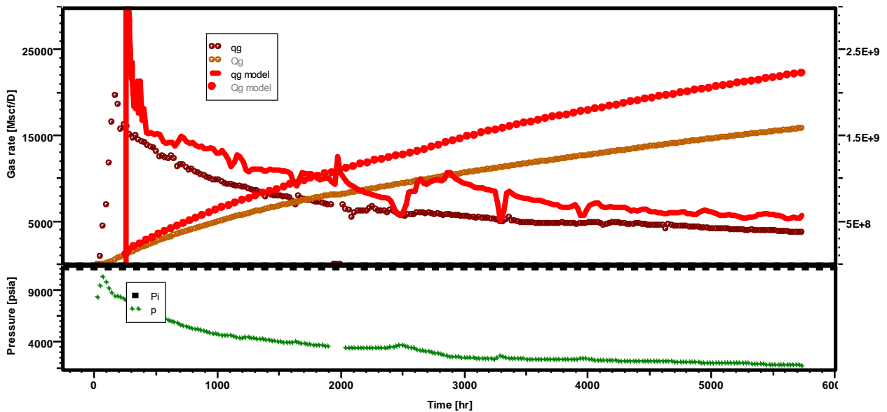
History match with the numerical model before refinement
