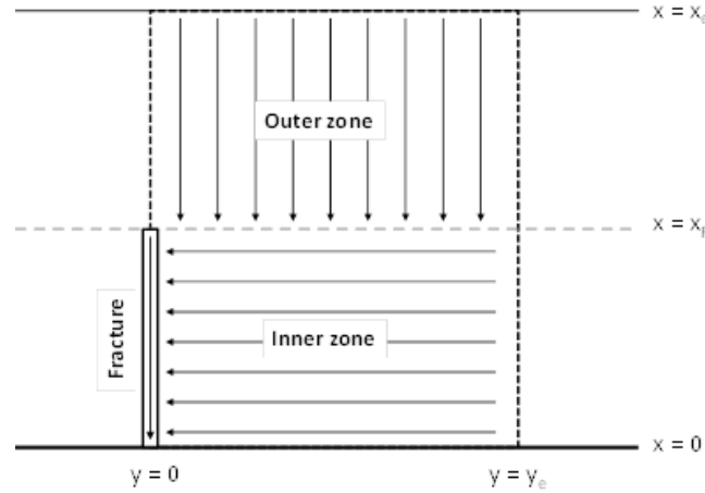
Fig. 1.H.6.33 - Tri-linear model basic component
