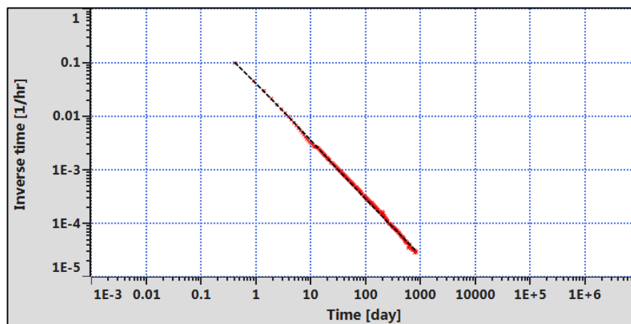
Fig. 1.D.8 – Rate/cumulative production and time plot (modified hyperbolic relation). (From Ilk, 2014)
