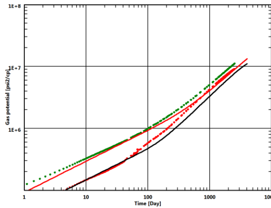
Fig. 1.E.11 – Loglog plot before adjustment.
