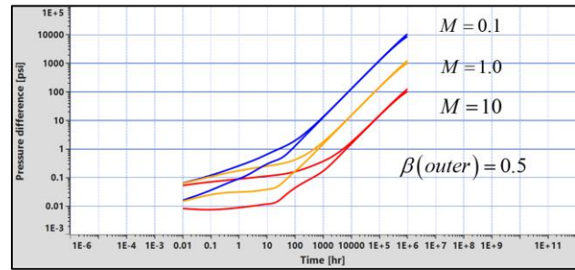
Fig. 1.H.6.48 - Closed outer zone, influence of mobility ratio with \beta=0.5
