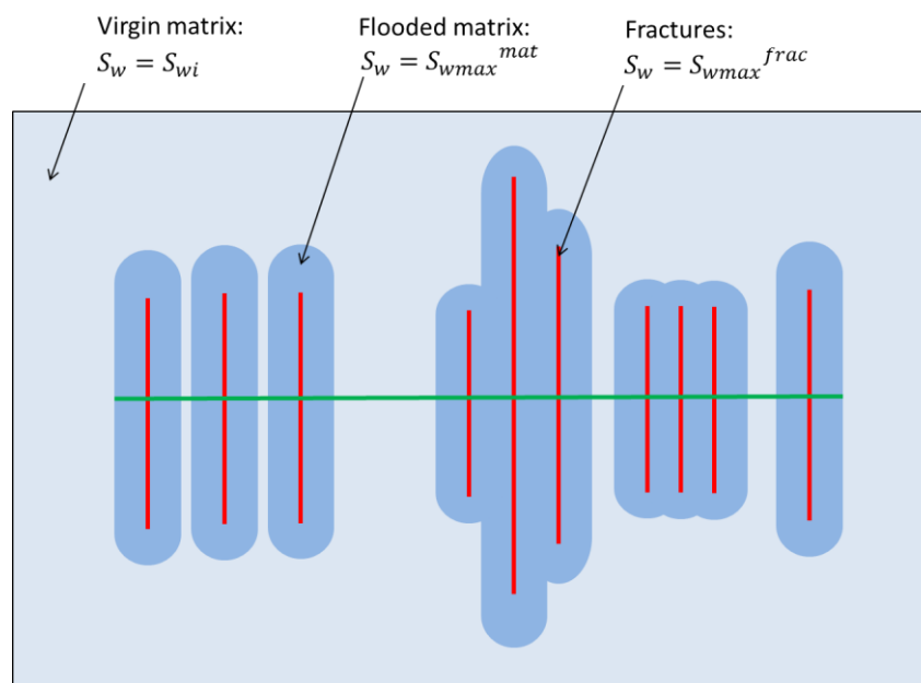
Fig. 1.B.14 – Initialization using the material balance static approach.
