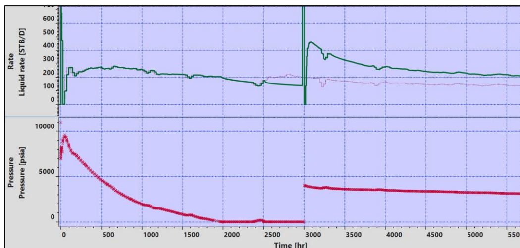
Fig. 1.H.22 - Pressure and rate history with two refrac jobs
