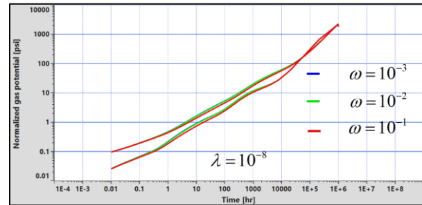
Fig. 1.H.6.56 - Closed outer zone, storativity ratio
