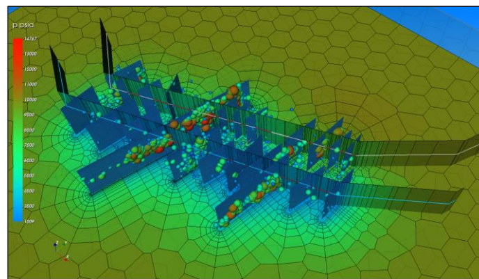
Fig. 1.H.13 – DFN constrained by seismic events
