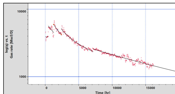
Fig. 1.D.30 – Segmented Hyperbolic DCA model match
