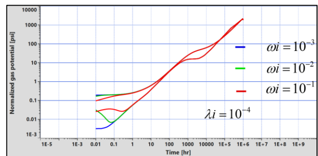
Fig. 1.H.6.54 - Closed outer zone, storativity ratio with \lambda = 0.0001
