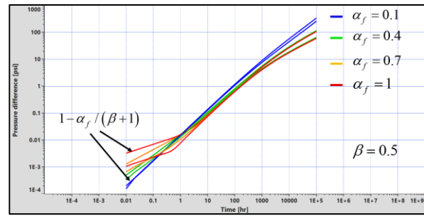
Fig. 1.H.6.40 - Influence of the inner zone \alpha (with \beta=0.5 )
