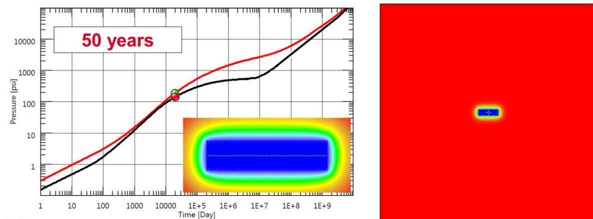
Fig. 1.C.5 – Deviation from the SRV flow
