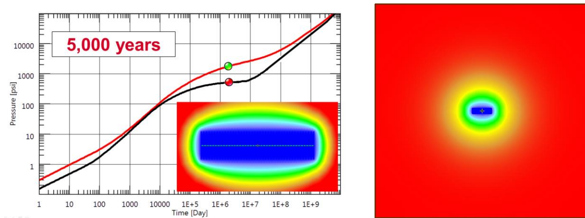
Fig. 1.C.7 – Possible IARF from the formation
