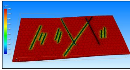
Fig. 1.H.24 - Pressure map after 3000 hr, refrac of "fracture 6"
