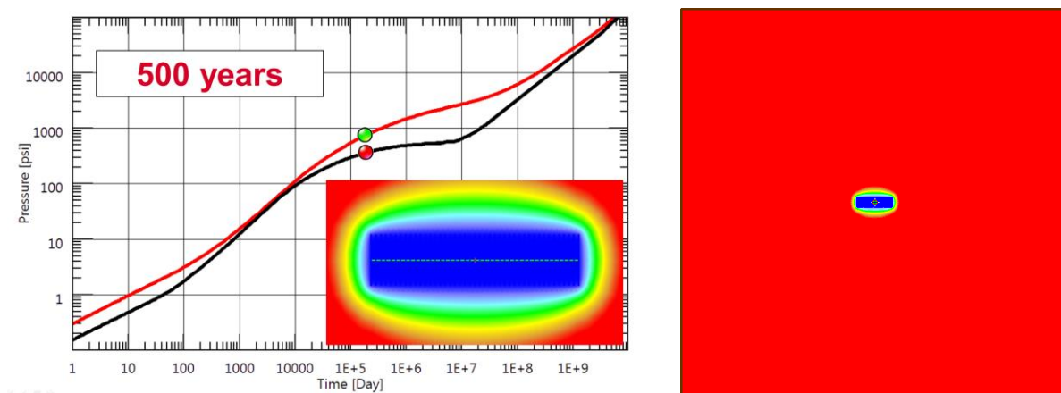
Fig. 1.C.6 – Effect of the formation out of SRV
