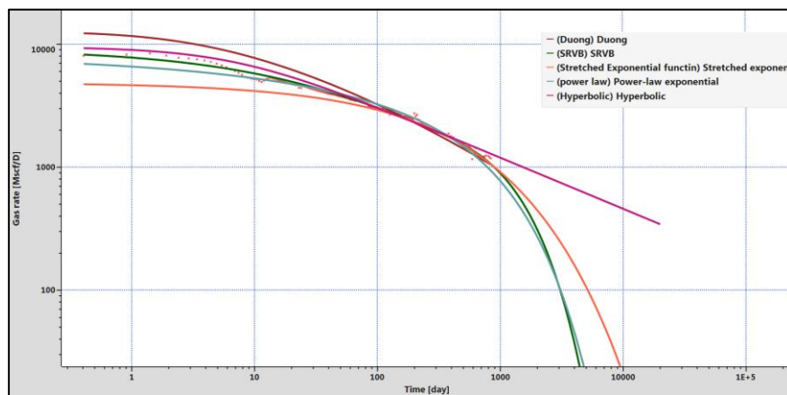
Fig. 1.D.32 – Rate and time plot (match with all models).
