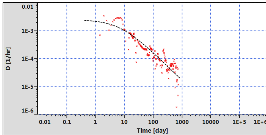
Fig. 1.D.6 – Computed D-parameter and time plot (modified hyperbolic relation).
