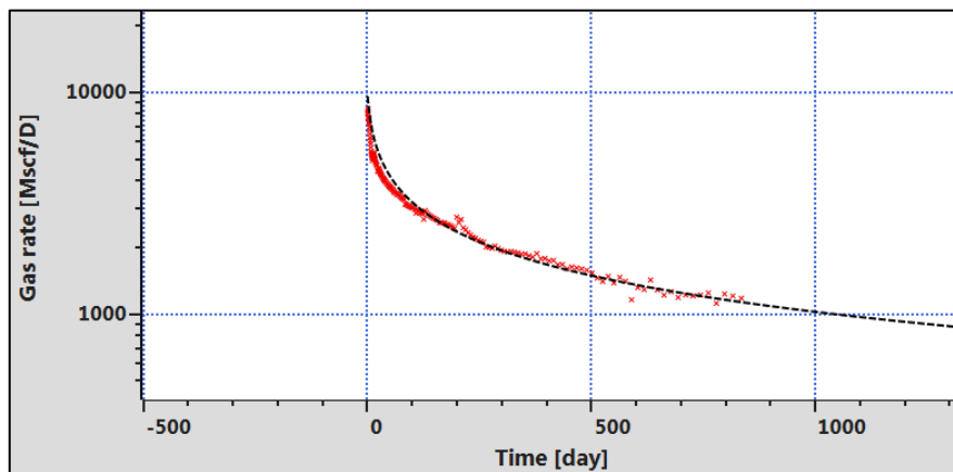
Fig. 1.D.17 – Rate and time plot (Duong model).
