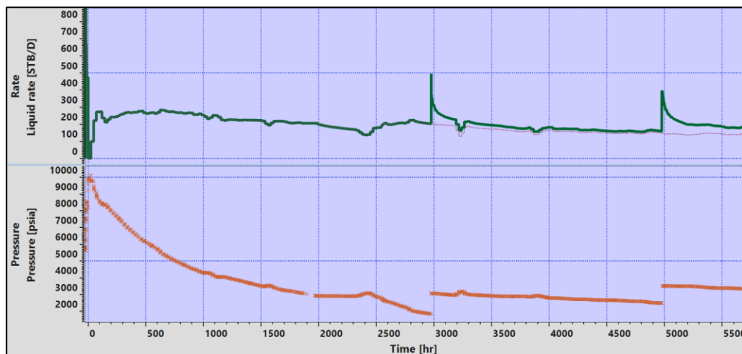
Fig. 1.H.26 - Pressure and rate history with two refrac jobs
