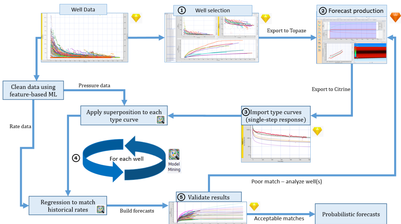
Fig. 1.I.11 – Diagram of the Model Mining workflow
