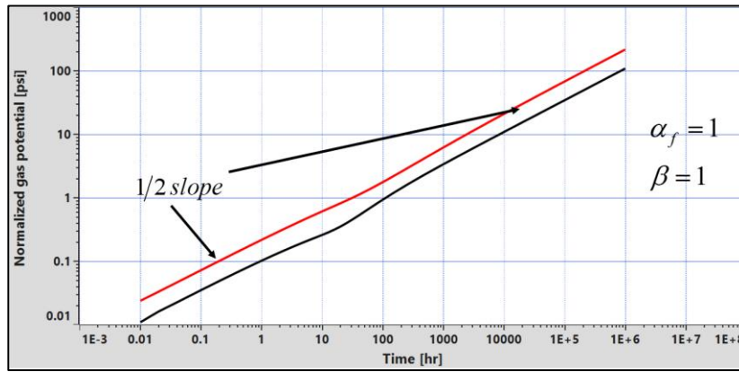
Fig. 1.H.6.34 - Reference case: 2 equal homogeneous regions, Infinite outer zone
