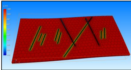
Fig. 1.H.23 - Pressure map before re-frac job
