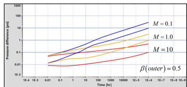
Fig. 1.H.6.46 - Infinite outer zone, influence of mobility ratio with \beta=0.5
