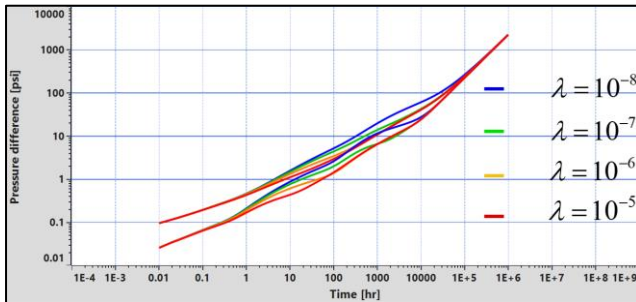
Fig. 1.H.6.55 - Closed outer zone, influence of interporosity flow coefficient with \omega=0.1
