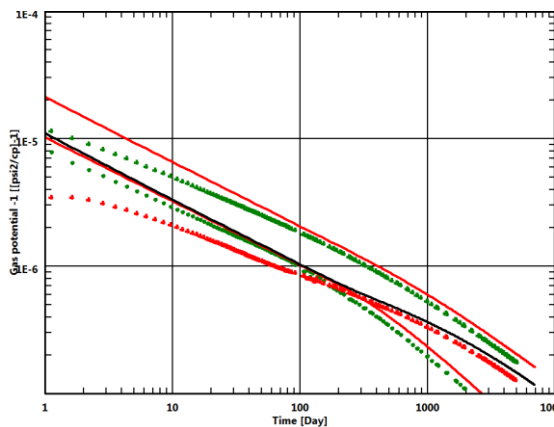
Fig. 1.E.13 – Blasingame plot before adjustment.
