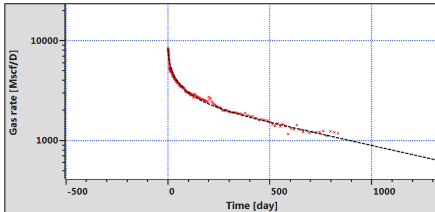
Fig. 1.D.25 – Rate and time plot (SVRB model).
