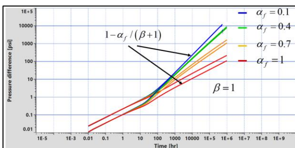
Fig. 1.H.6.37 - Influence of the outer zone \alpha (constant \beta=1 )
