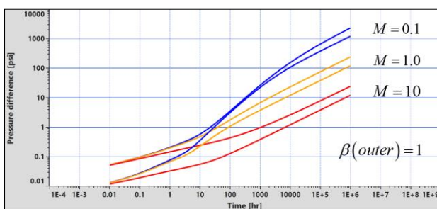
Fig. 1.H.6.45 - Infinite outer zone, influence of mobility ratio with \beta=1
