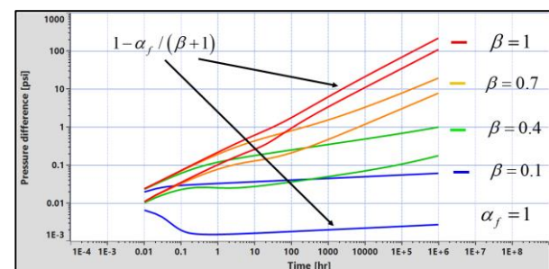
Fig. 1.H.6.38 - Influence of the outer zone \beta (constant \alpha=1 )
