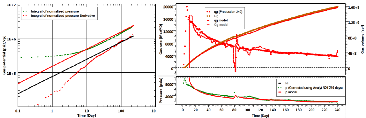
Fig. 1.G.3 – Match with a single fracture model on the Loglog and history plots.
