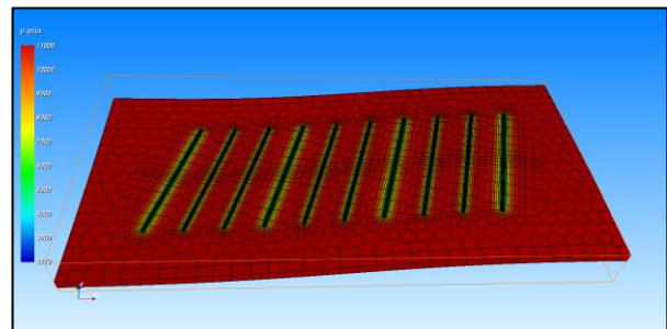
Fig. 1.H.21 - Pressure map after re-frac job
