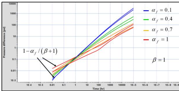
Fig. 1.H.6.39 - Influence of the inner zone \alpha (with \beta=1 )
