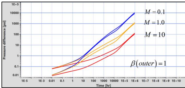
Fig. 1.H.6.47 - Closed outer zone, influence of mobility ratio with \beta=1
