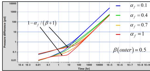
Fig. 1.H.6.44 - Closed outer zone, influence of \alpha (with \beta=0.5 )
