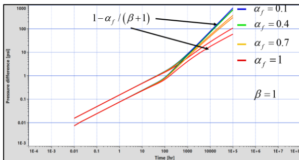
Fig. 1.H.6.41 - Influence of the outer zone \alpha (with \beta=1 )
