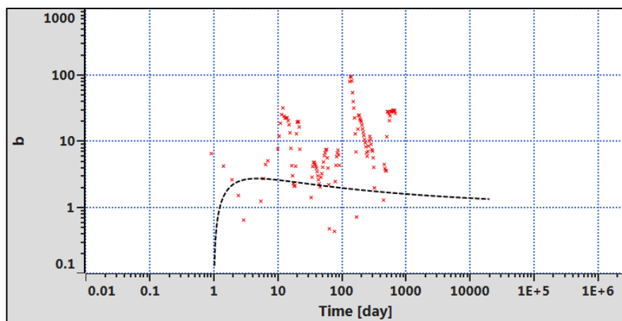
Fig. 1.D.19 – Computed b-parameter and time plot (Duong model).
