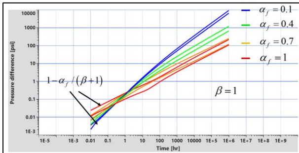
Fig. 1.H.6.35 - Influence of the inner zone \alpha (constant \beta=1 )
