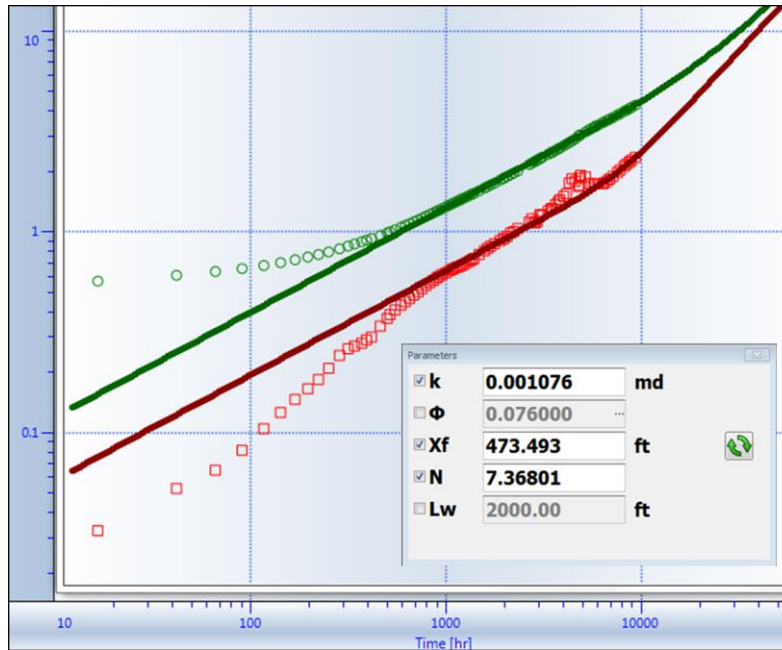
Fig. 1.F.6 – Using the SRV model as a diagnostic tool .
