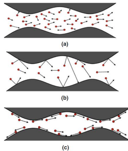
Fig. 1.B.3 – Schematic of cross section of a pore and gas molecule:
