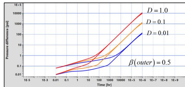
Fig. 1.H.6.50 - Closed outer zone, influence of diffusivity ratio with \beta=0.5
