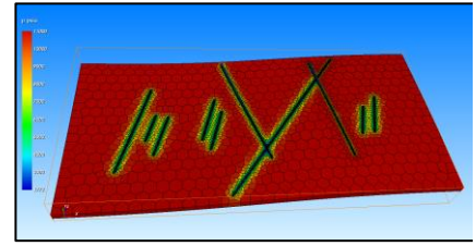
Fig. 1.H.25 - Pressure map after 5000 hr, refrac of "fracture 8"
