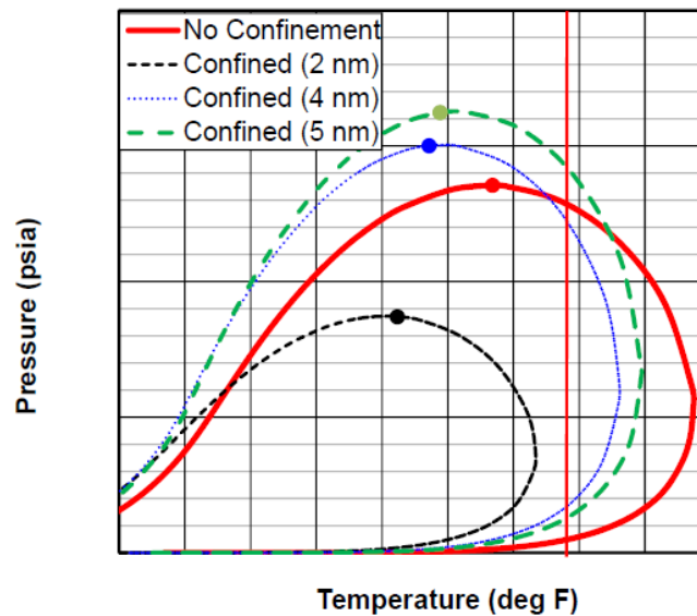
Fig. 1.B.12 – Phase diagrams of confined and unconfined gas-condensate fluid. (From Devegowda et al, 2012)
