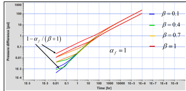
Fig. 1.H.6.36 - Influence of the inner zone \beta (constant \alpha=1 )
