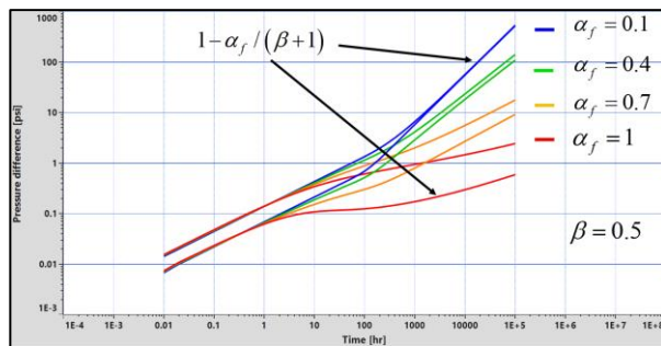
Fig. 1.H.6.42 - Influence of the outer zone \alpha (with \beta=0.5 )
