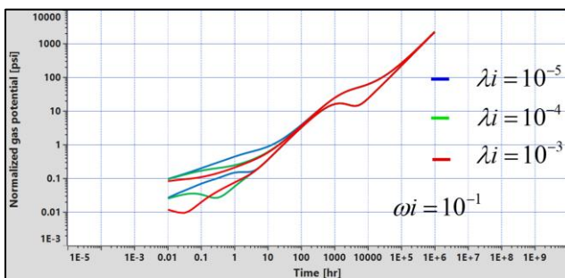
Fig. 1.H.6.53 - Closed outer zone, influence of interporosity flow coefficient with \omega = 0.1
