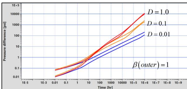
Fig. 1.H.6.49 - Closed outer zone, influence of diffusivity ratio with \beta=1
