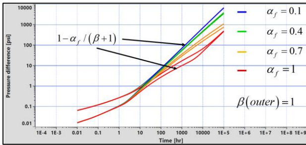
Fig. 1.H.6.43 - Closed outer zone, influence of \alpha (with \beta=1 )
