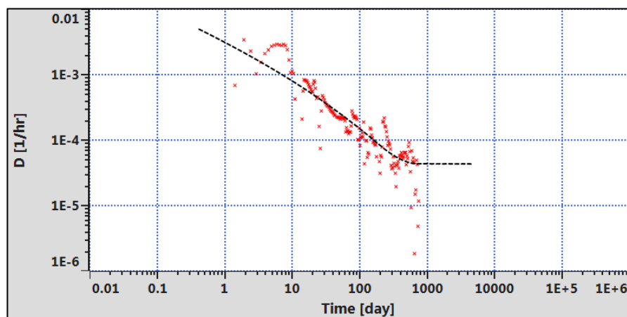
Fig. 1.D.26 – Computed D-parameter and time plot (SVRB model).
